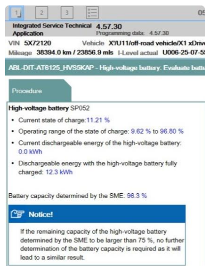
3.1 Test HV-Battery condition OK, 96,3 %
